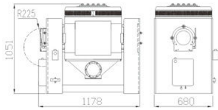
Shaker ET-20-445
