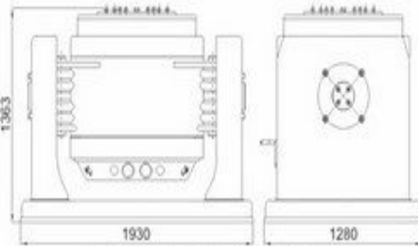
Shaker ET-100/120-550
