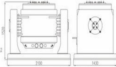
Shaker ET-160/180-590
